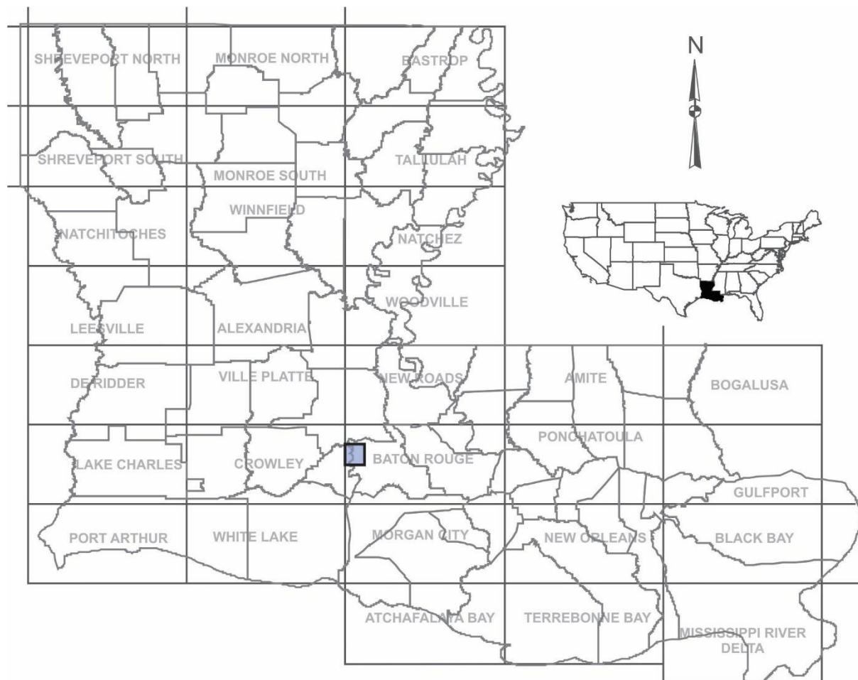
1. Location of Breau Bridge 7.5-minute quadrangle, southeastern Louisiana.
